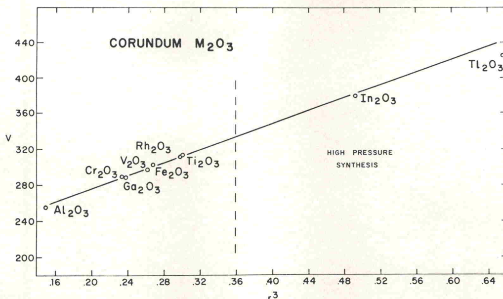
Figure 6.—Corundum unit cell volumes vs. effective cation volume ( r_e^3 ).
