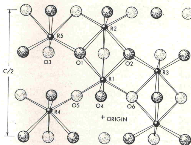
Figure 3.—The corundum structure viewed along an a axis of the hexagonal cell (after Newnham and de Haan 7 ).
