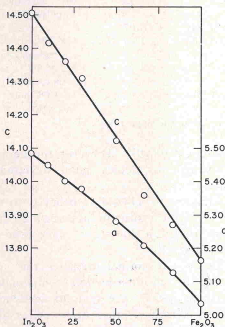
Figure 2.—Cell dimensions for the \text{In}_2\text{O}_3 - \text{Fe}_2\text{O}_3 system quenched from 65 kbars.
